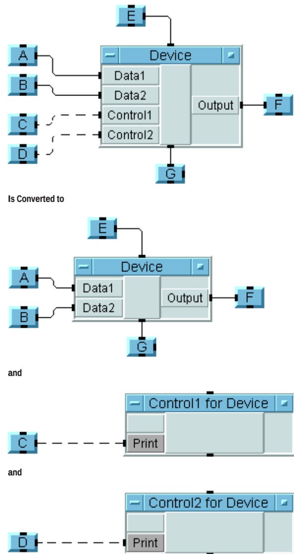
Figure 12 Expansion of control pins.
